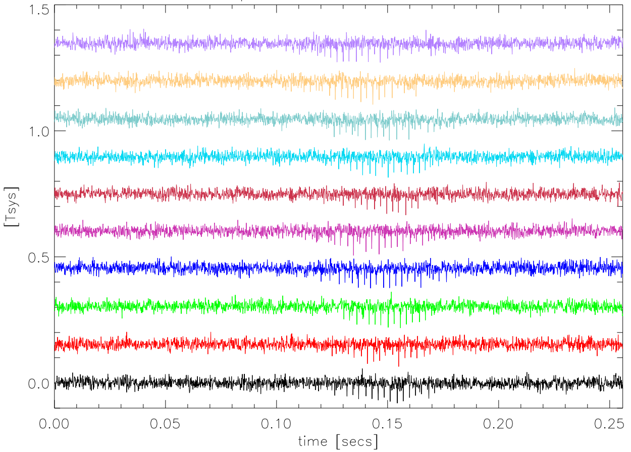
30nov05 Alfa compression with 100Mhz filter in Beam:1B
