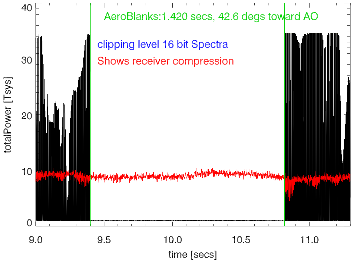
blowup around aerostat blanking toward AO
