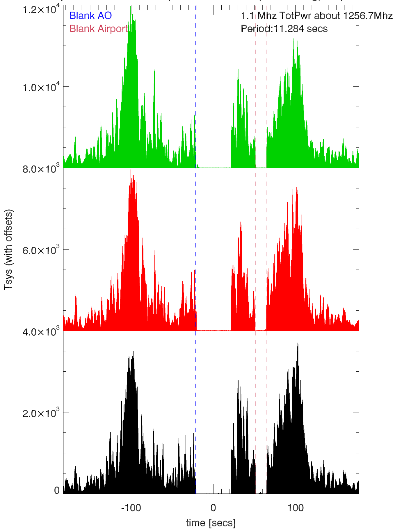
22apr14 Aerostat total pwr vs azimuth (AO=0deg). 3 periods
