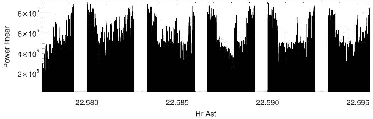
2130 02nov11 totPwr vs Tm (65secs). puntaSalinas freq:1258.3 Mhz
