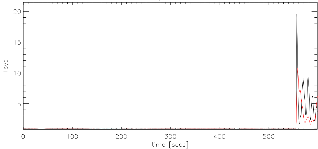
20090207 scan:903800066 peak value 1380.3–1381.5 vs time
