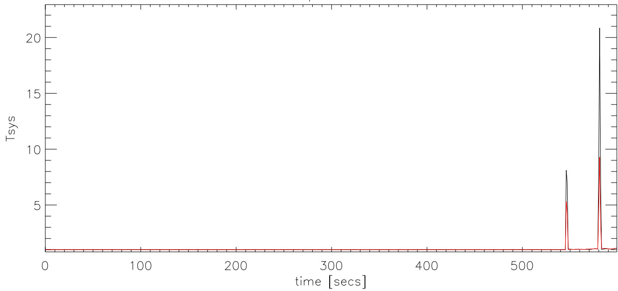
20090120 scan:902000038 peak value 1380.3–1381.5 vs time
