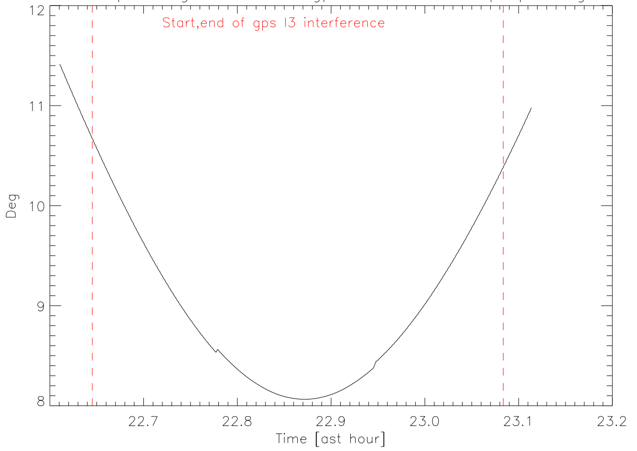
27sep10 angular distance gps svn and telescope pointing
