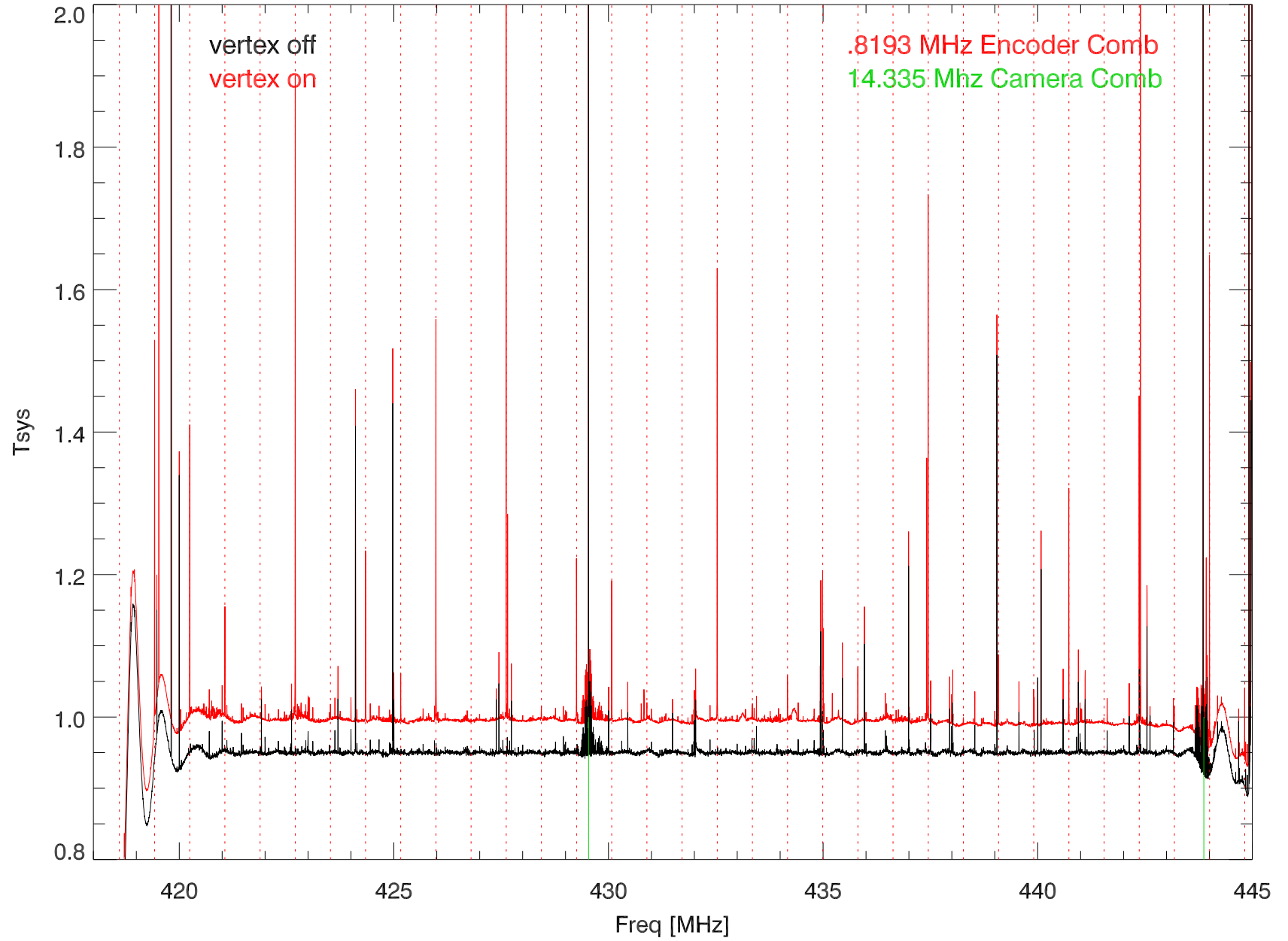
180611 430Rcvr avgSpectra vertex off, vertex on.
