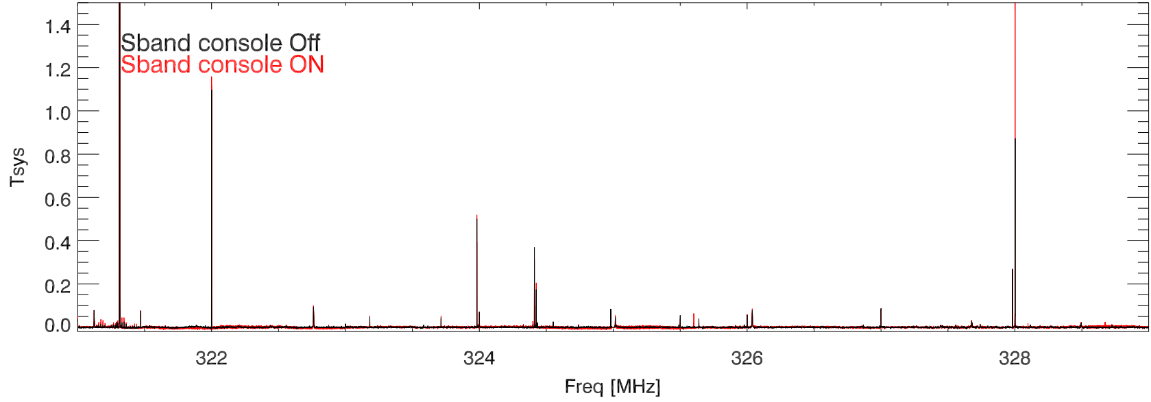
01jun17 327 rcvr. sband console on, off(afterRepairs) bm3
