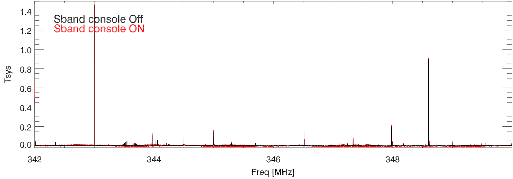
01jun17 327 rcvr. sband console on, off(afterRepairs) bm6
