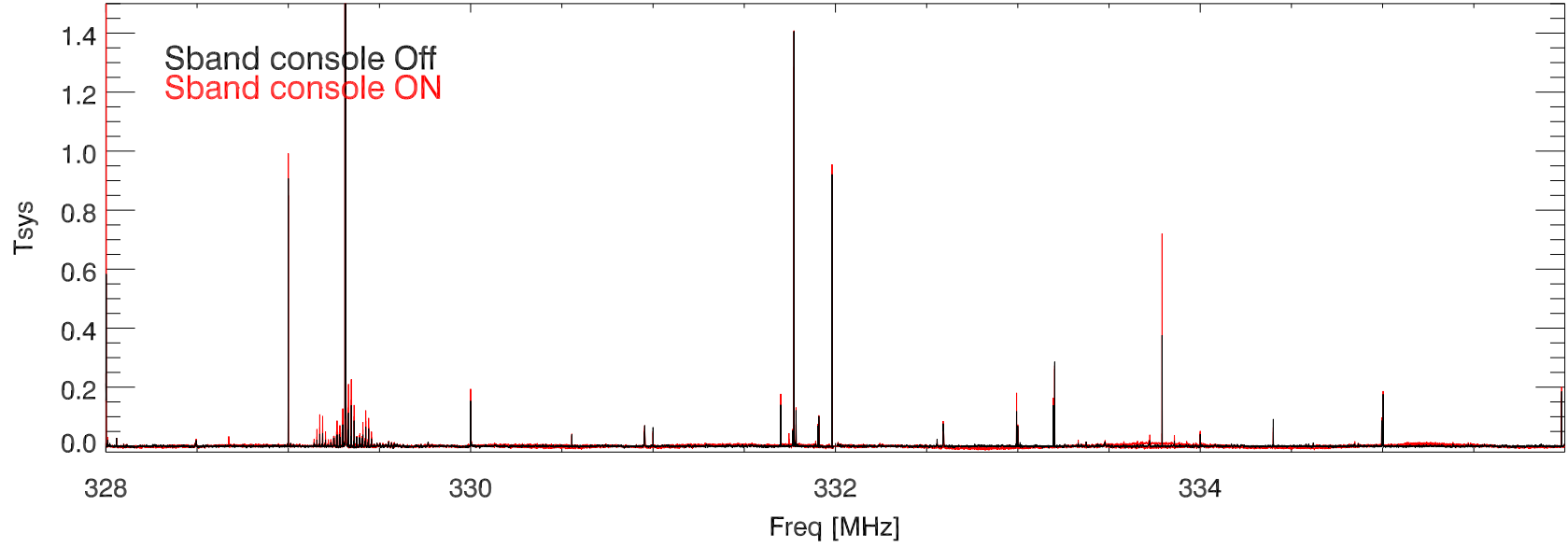
01jun17 327 rcvr. sband console on, off(afterRepairs) bm4
