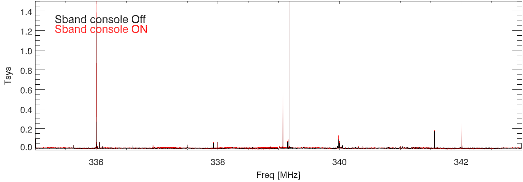
01jun17 327 rcvr. sband console on, off(afterRepairs) bm5
