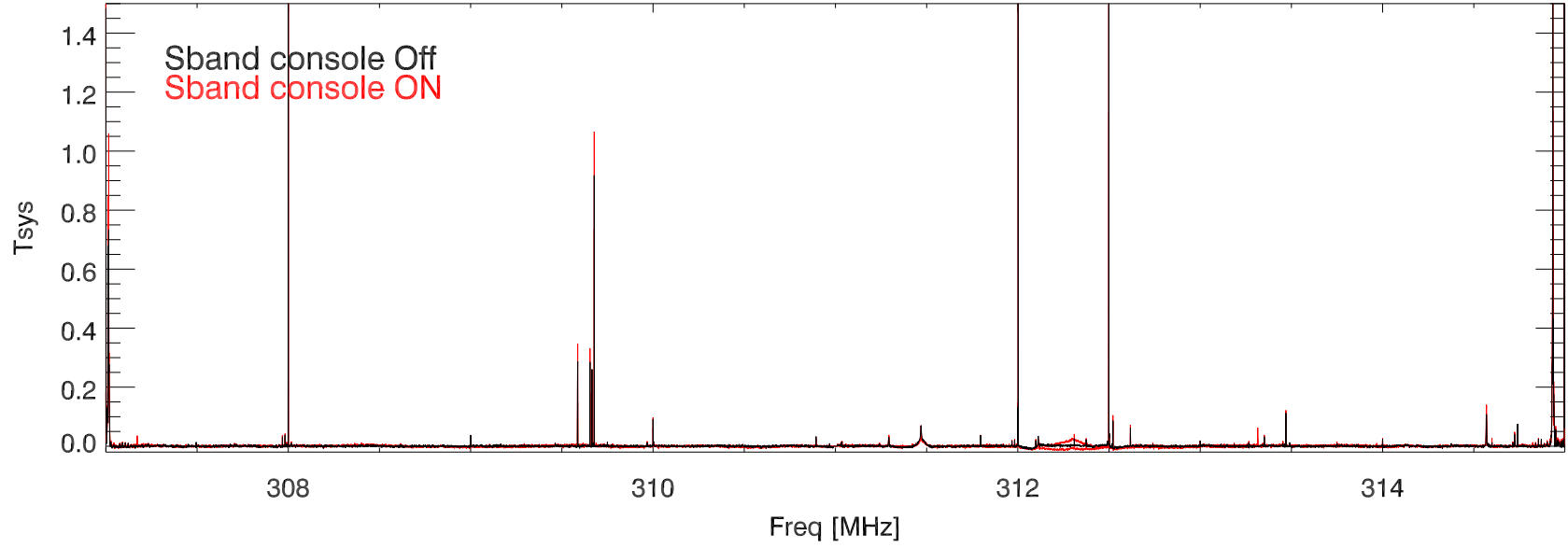
01jun17 327 rcvr. sband console on, off(afterRepairs) bm1
