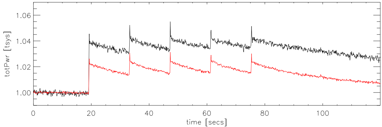
file 1000 beam 3: 3b stage 3. I [19 \rightarrow 15ma], dc block,isolator, before filter
