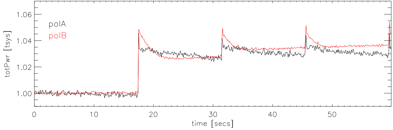
file 500 beam 3: normal settings
