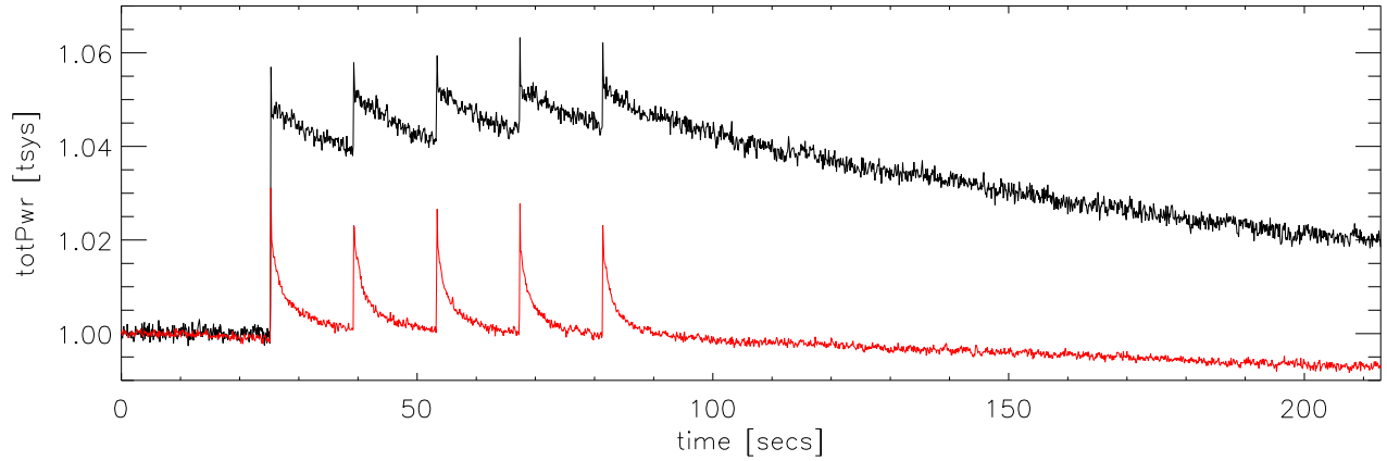
file 1100 beam 3: 3b stage 3. I [19 \rightarrow 22ma], dc block,isolator, before filter
