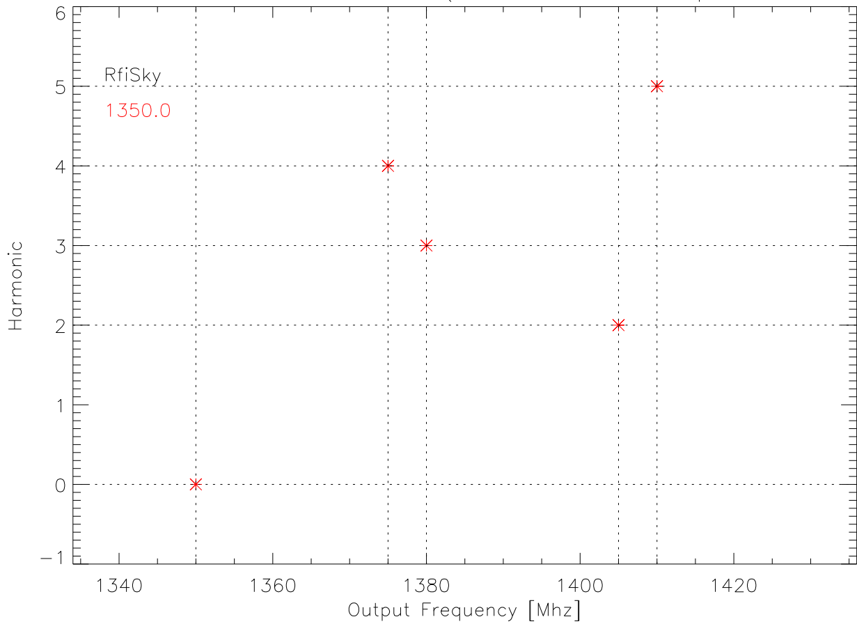
Harmonics of RFI in A2010 band (cfr=1385MHz, 250Bpfilter=110 Mhz)
