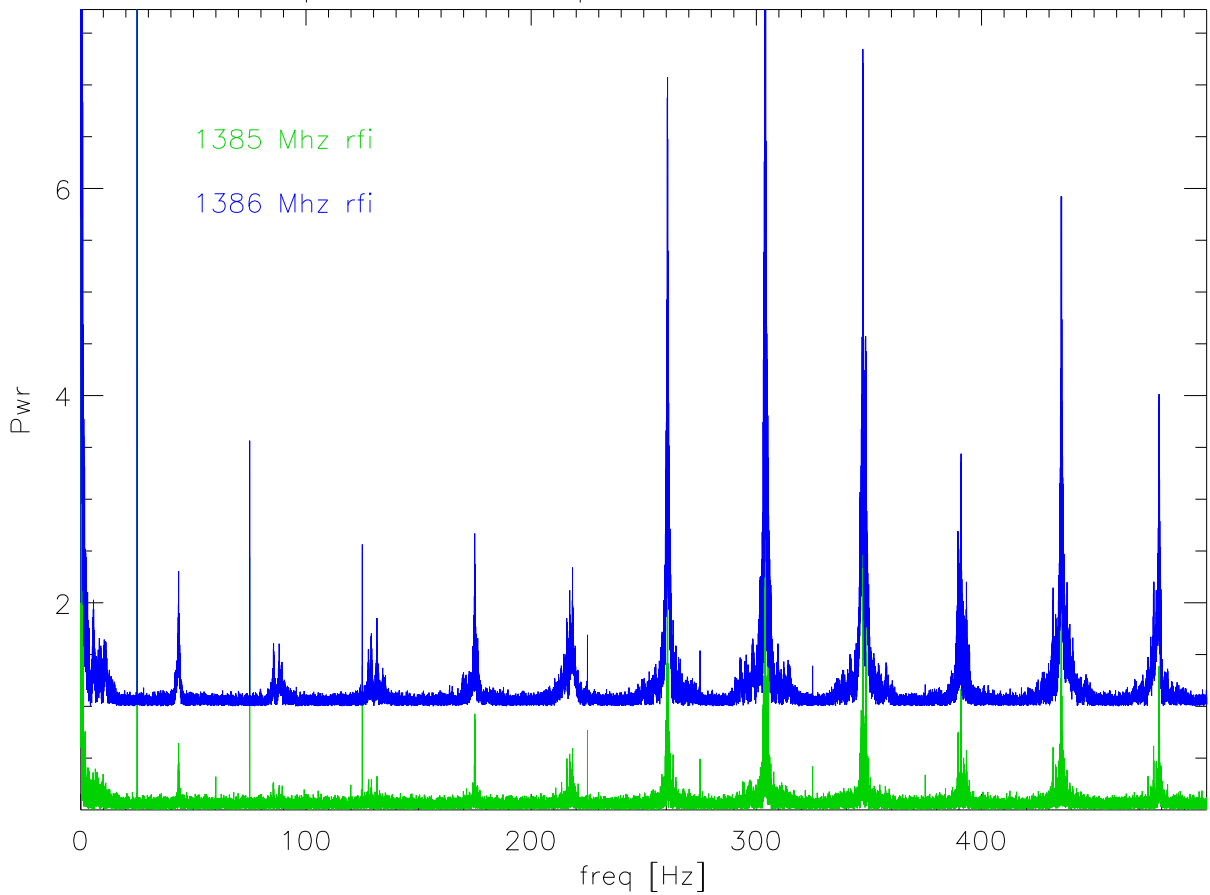
spectra of total power for 1385,1386 rfi
