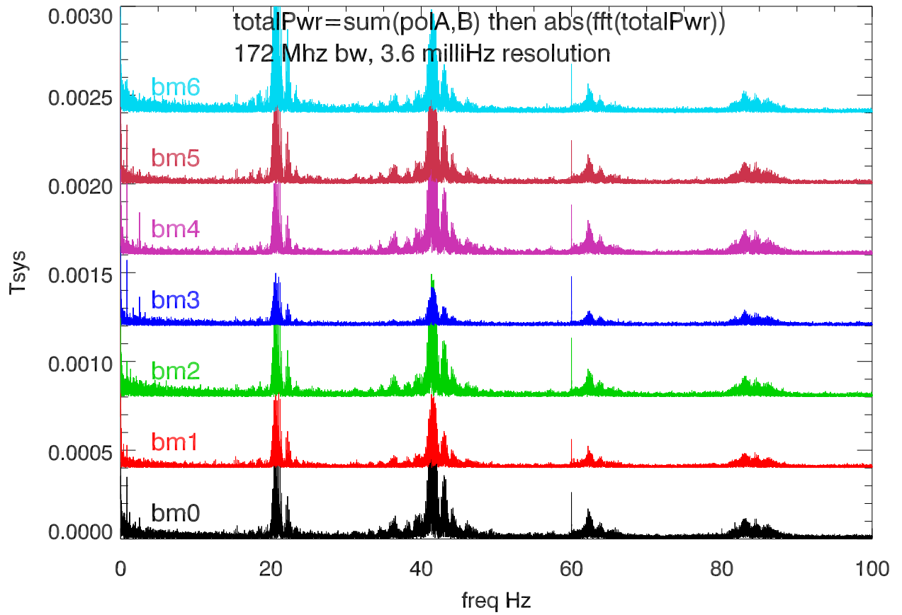
24may12 p2030 J1910+1017 spectra of total power. 1450 band
