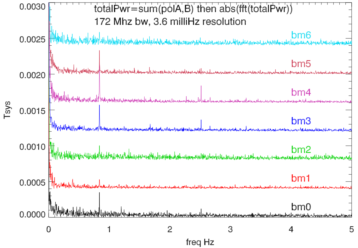
24may12 p2030 J1910+1017 spectra of total power. 1450 band
