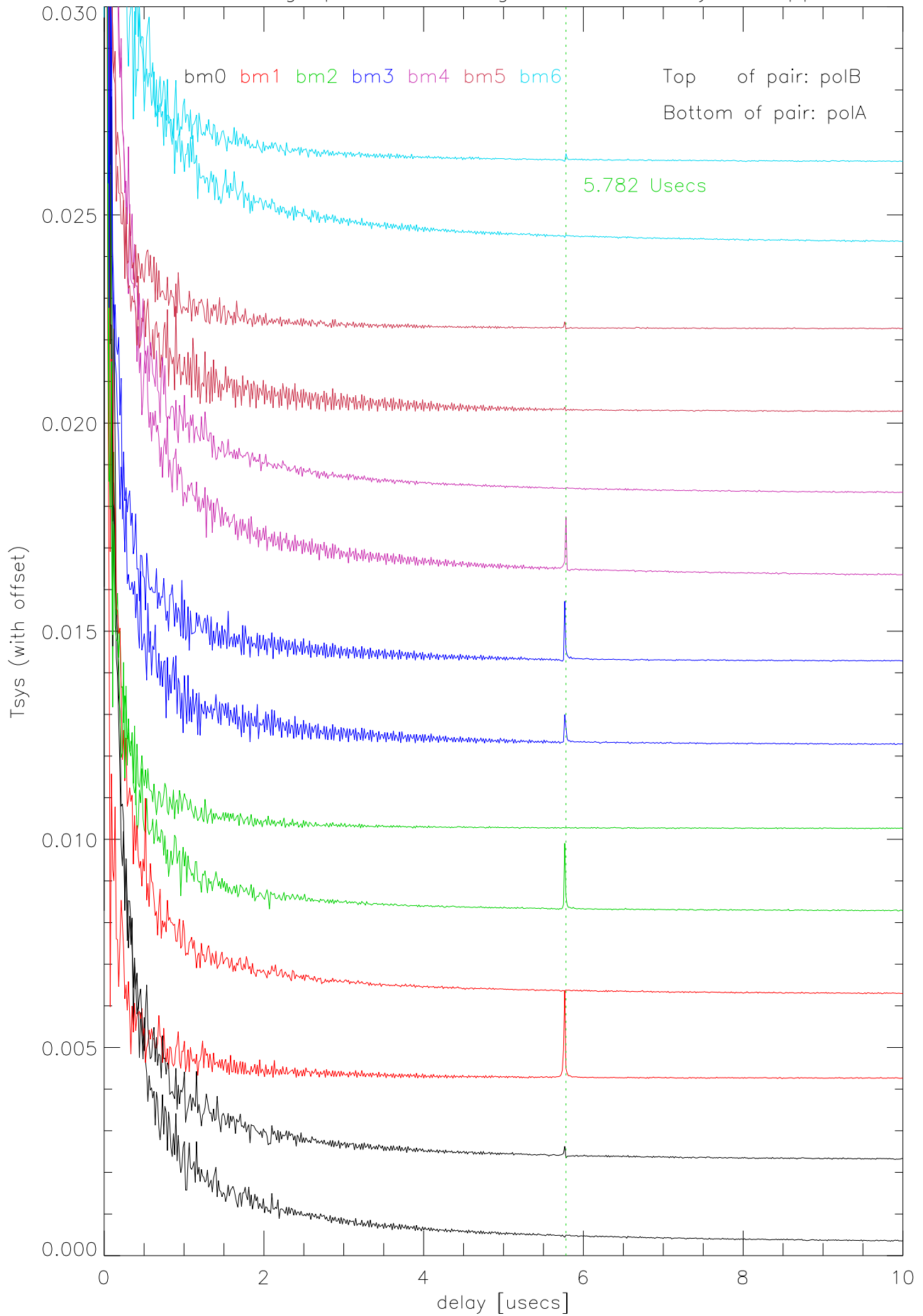
Acf of avg spectra showing reflection delay for ripple
