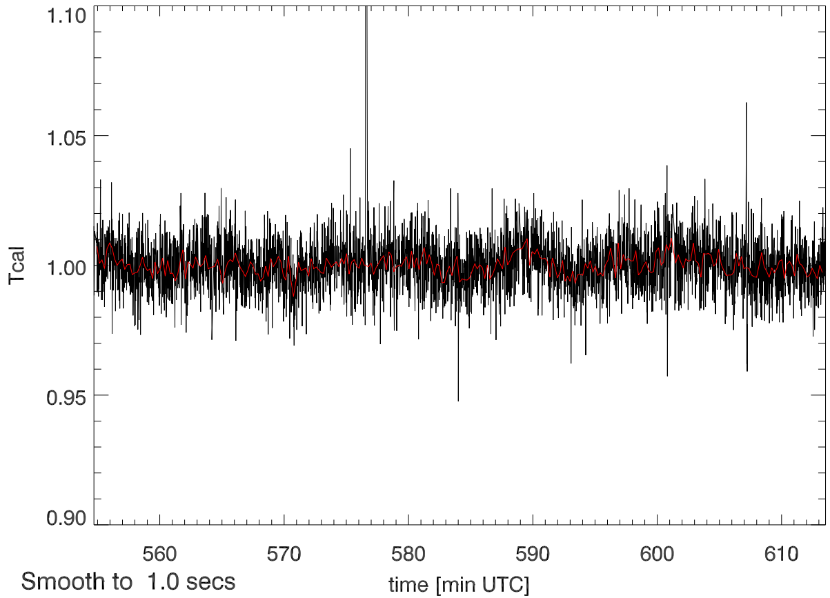
28nov15 calOn - calOff Beam6A SigA: 0.018
