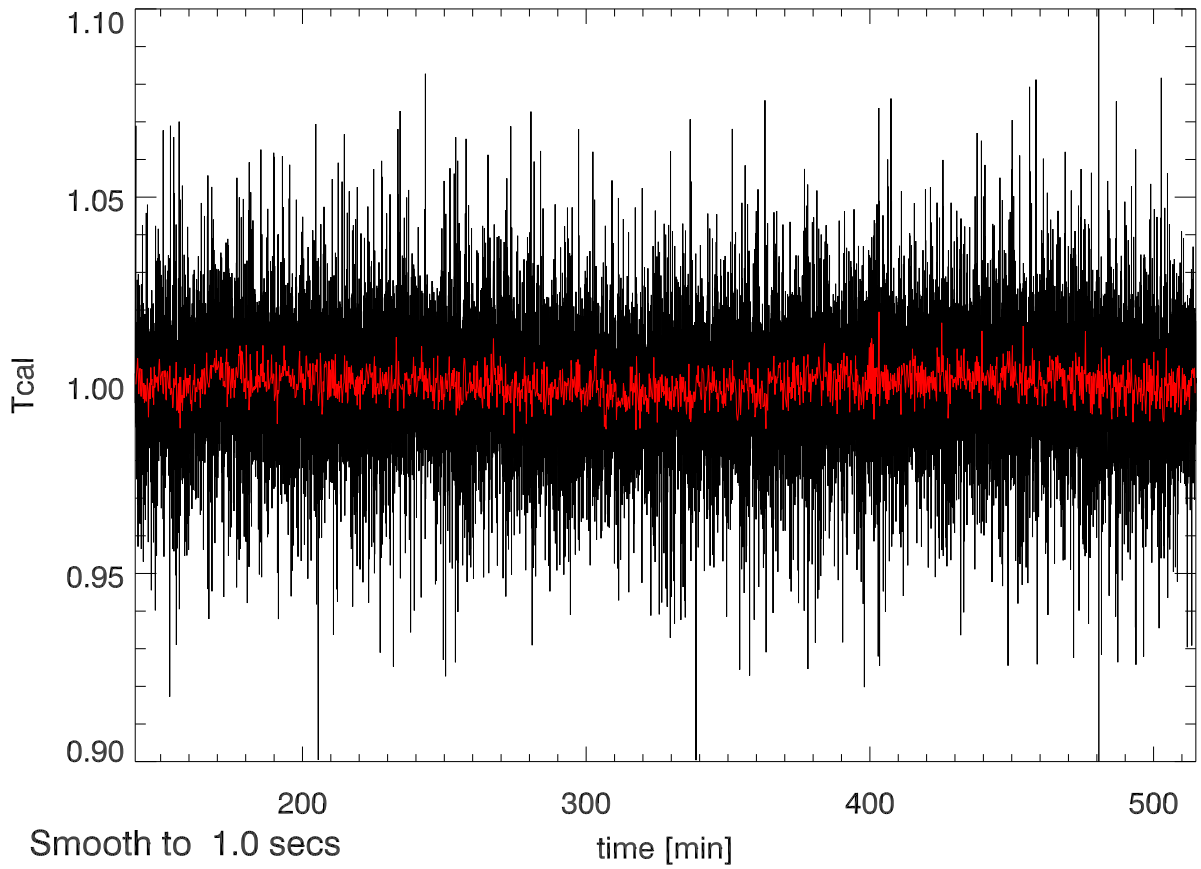
06may12 calOn - calOff Beam6A SigA: 0.028
