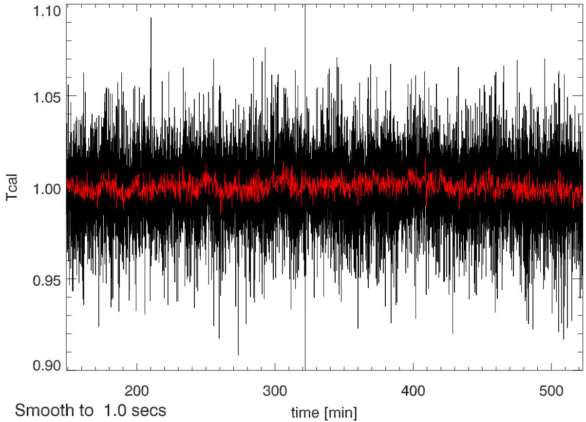
04may12 calOn - calOff Beam6A SigA: 0.028
