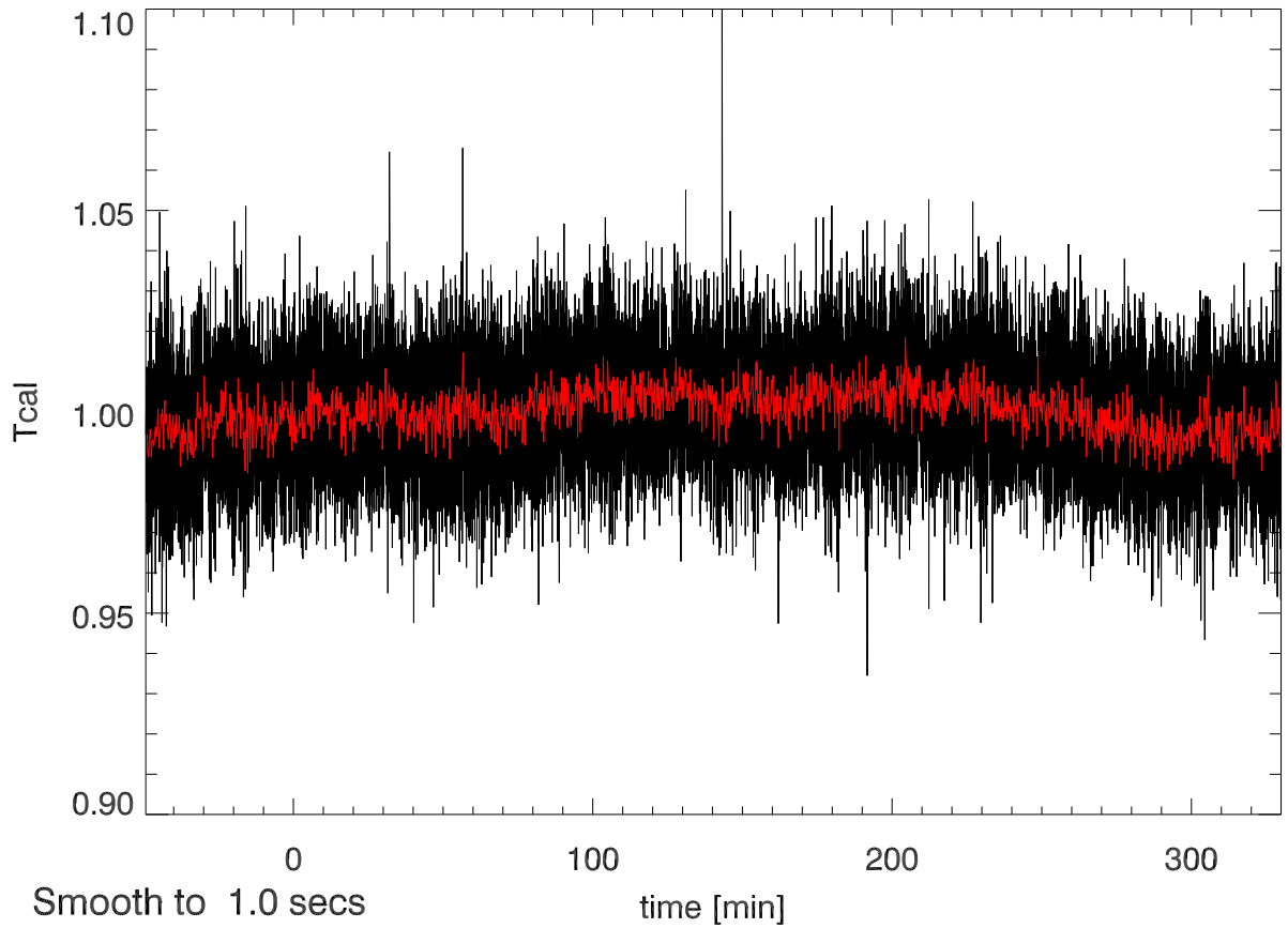
29oct11 calOn - calOff Beam5A SigA: 0.025
