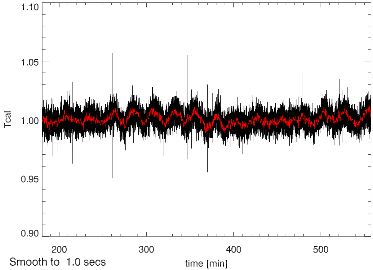
28jan13 calOn - calOff Beam5A SigA: 0.012
