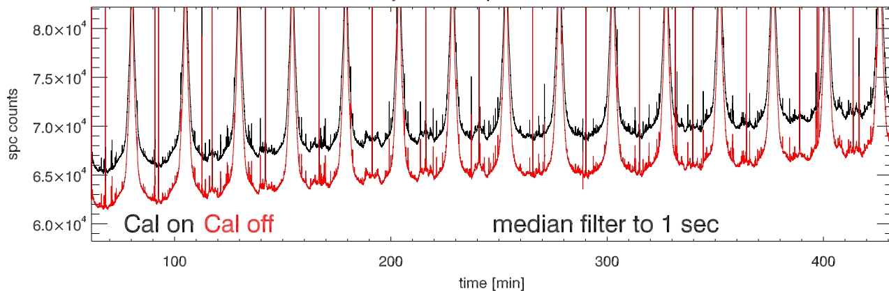
27may12 a2030 tp vs time. Beam5A
