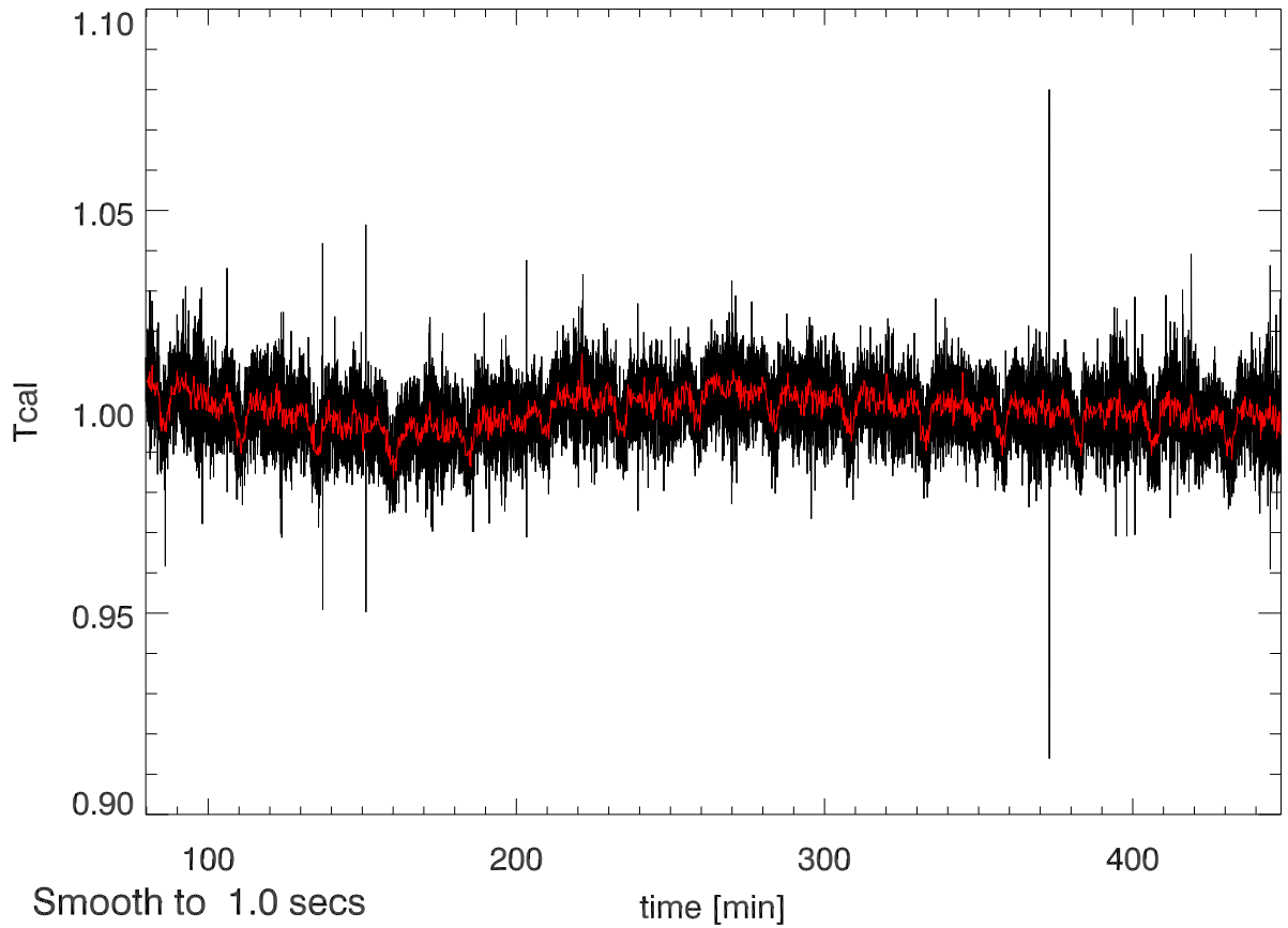
26feb13 calOn - calOff Beam5A SigA: 0.012
