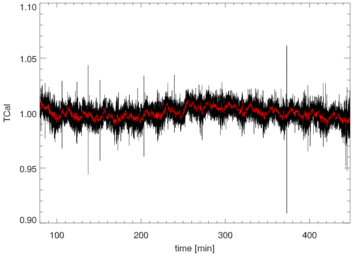
calOn - calOff Beam5B SigB: 0.011
