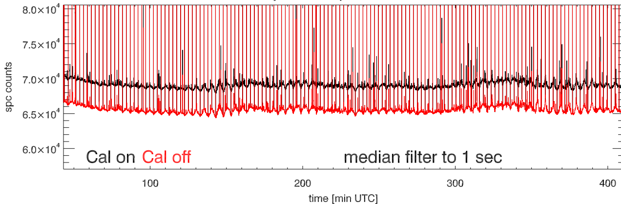
22may13 a2030 tp vs time. Beam5A
