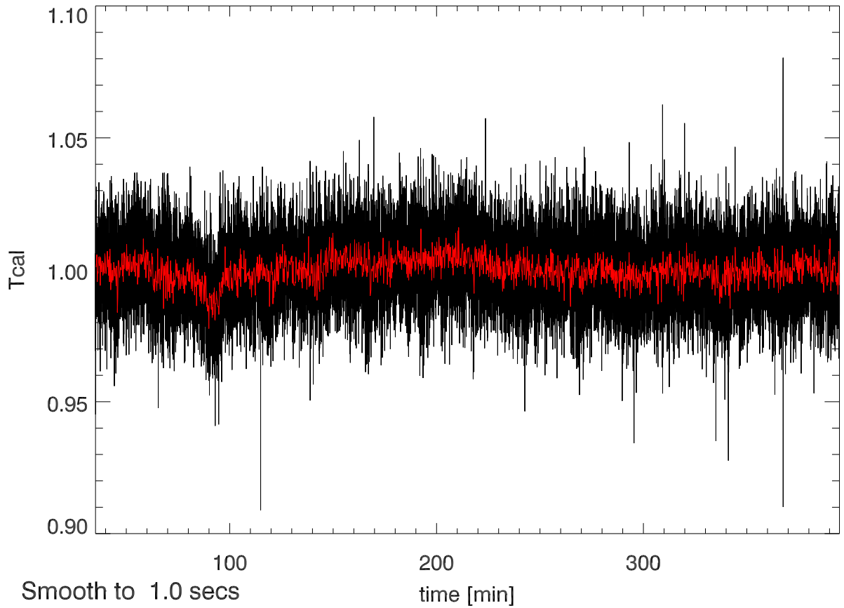
14apr11 calOn - calOff Beam5A SigA: 0.025
