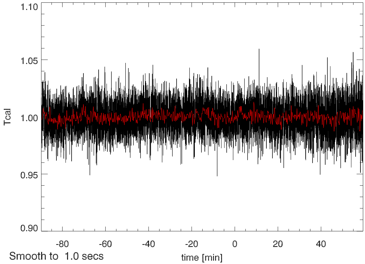
13nov11 calOn - calOff Beam5A SigA: 0.025
