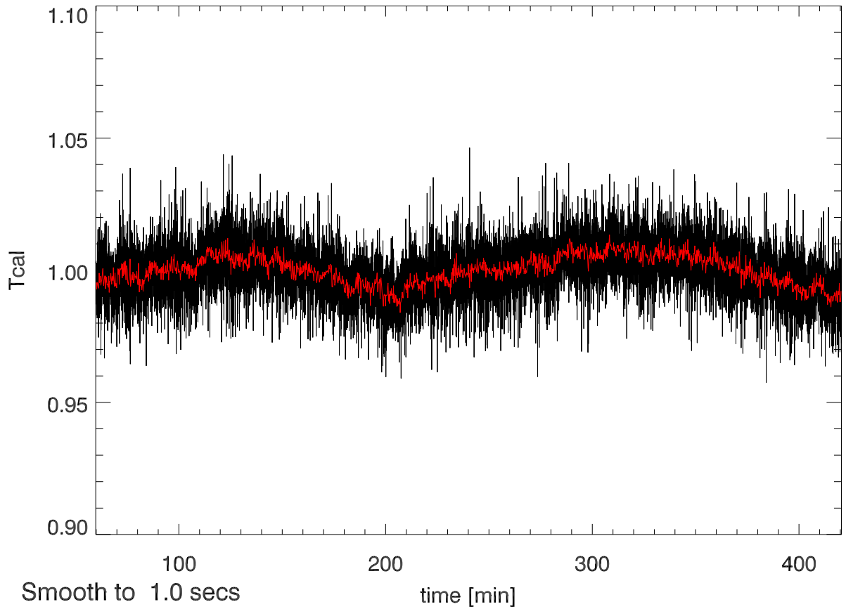
30may12 calOn - calOff Beam4A SigA: 0.015
