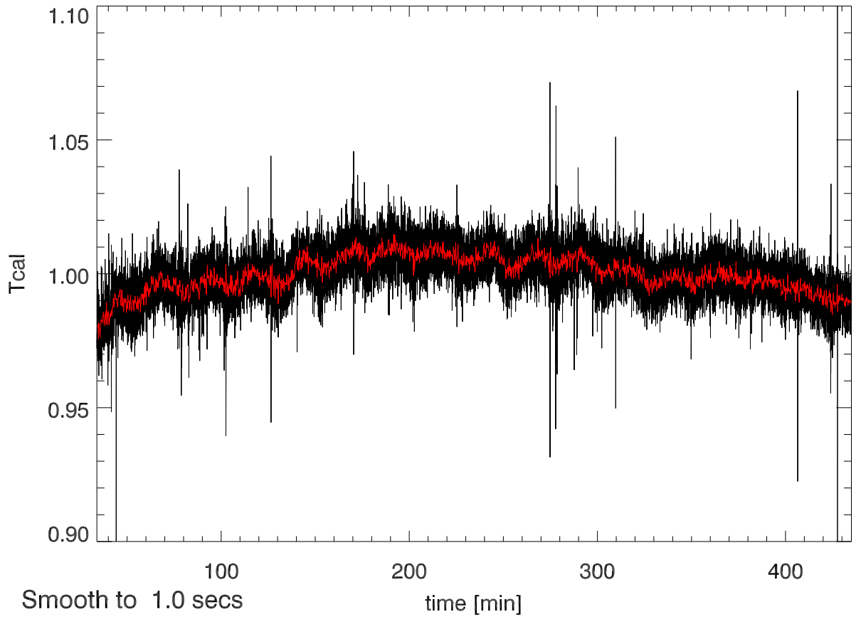
30aug12 calOn - calOff Beam4A SigA: 0.013
