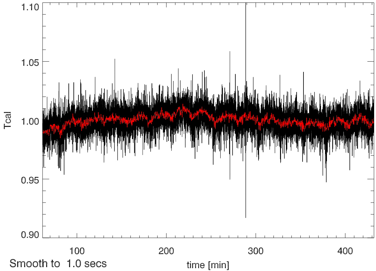
27may12 calOn - calOff Beam4A SigA: 0.015
