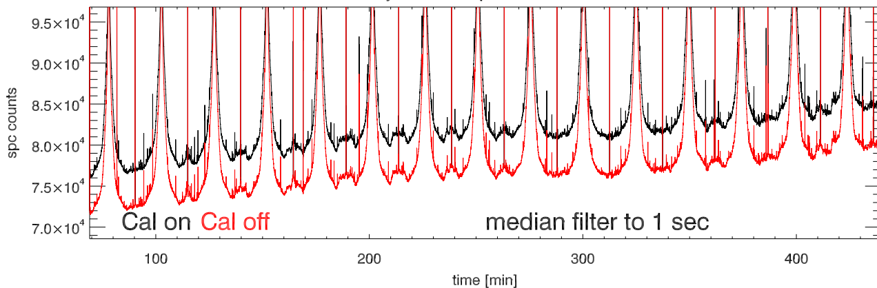
25may12 a2030 tp vs time. Beam4A
