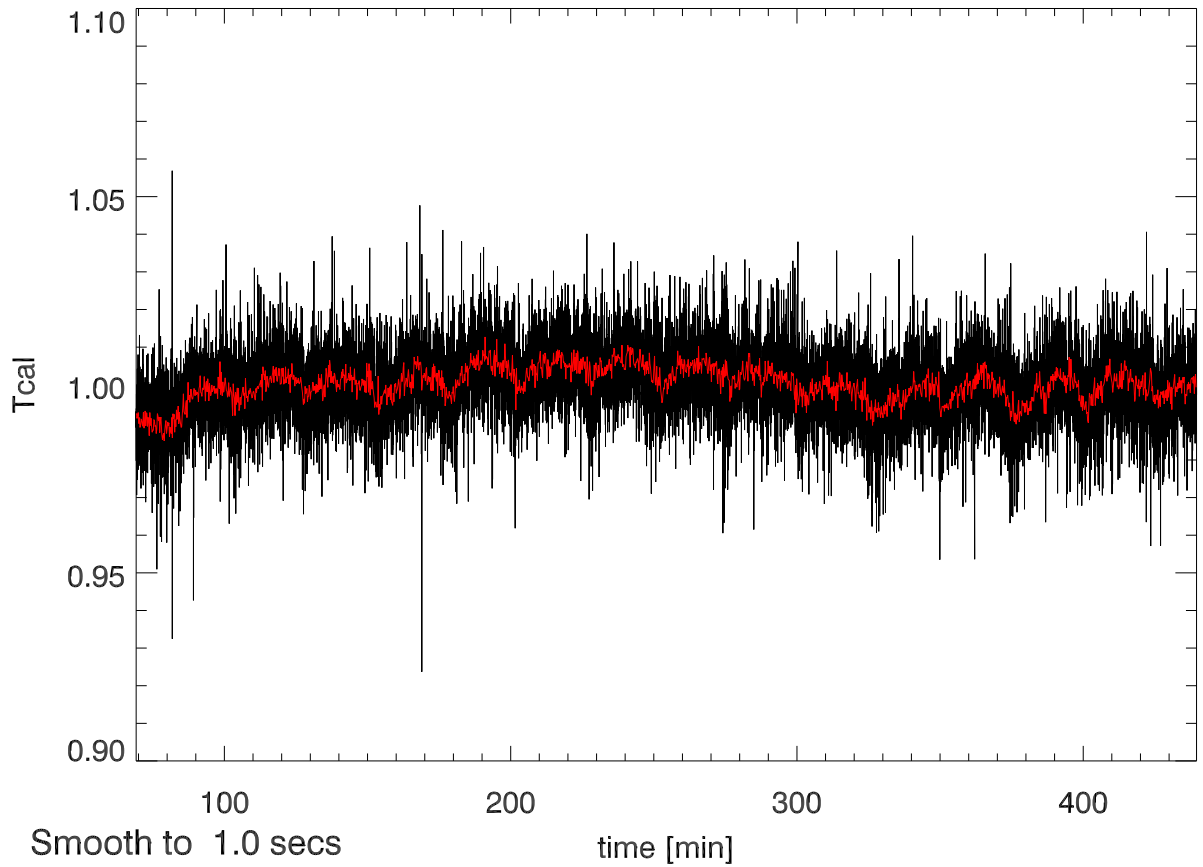
25may12 calOn - calOff Beam4A SigA: 0.015
