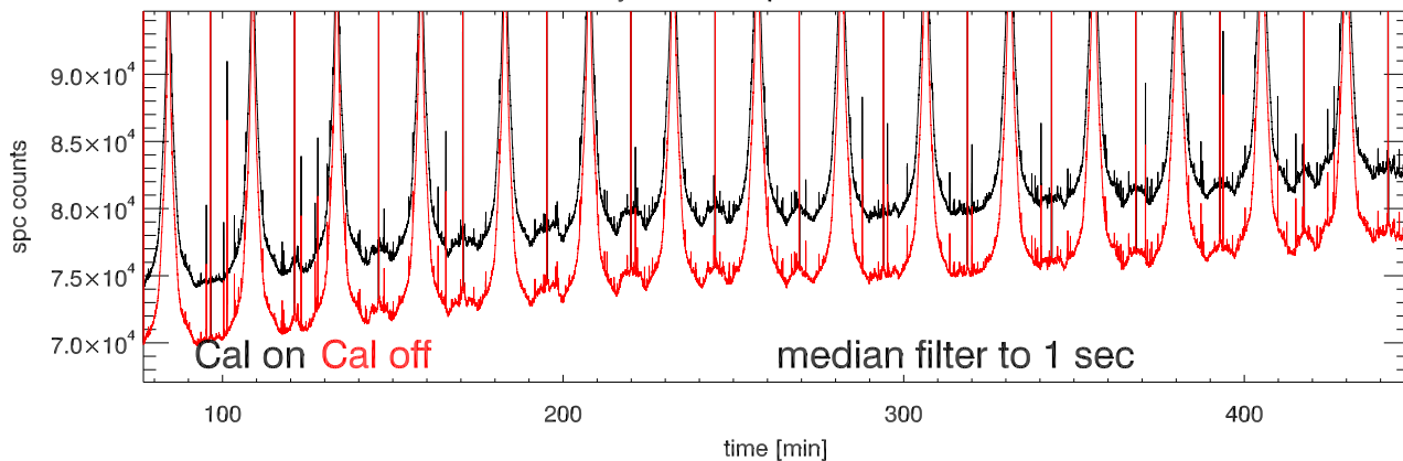
23may12 a2030 tp vs time. Beam4A
