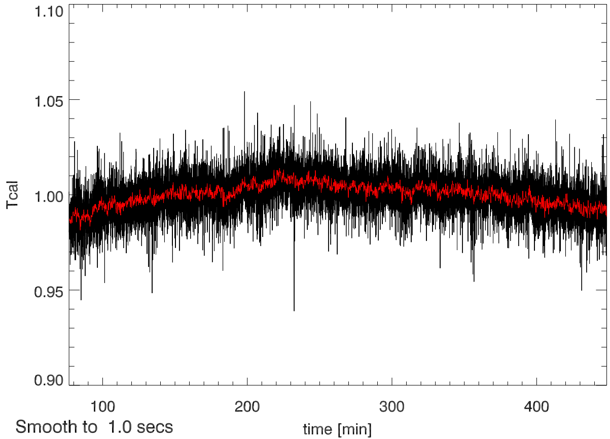
23may12 calOn - calOff Beam4A SigA: 0.015
