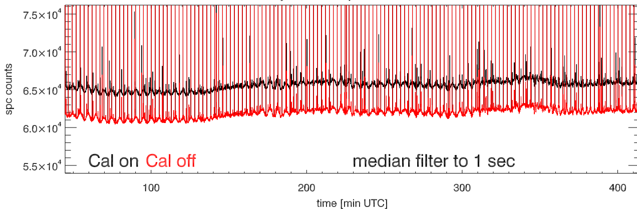
21may13 a2030 tp vs time. Beam4A
