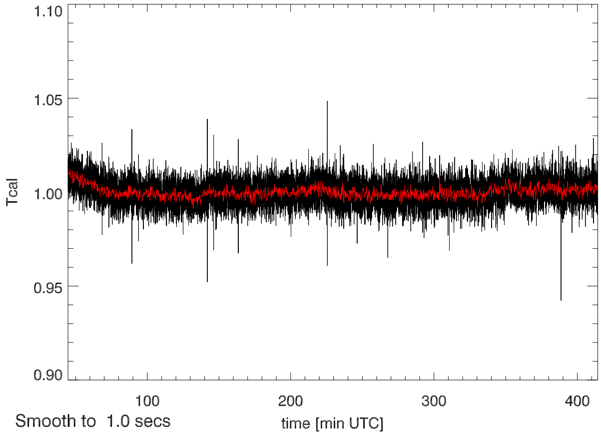
21may13 calOn - calOff Beam4A SigA: 0.011
