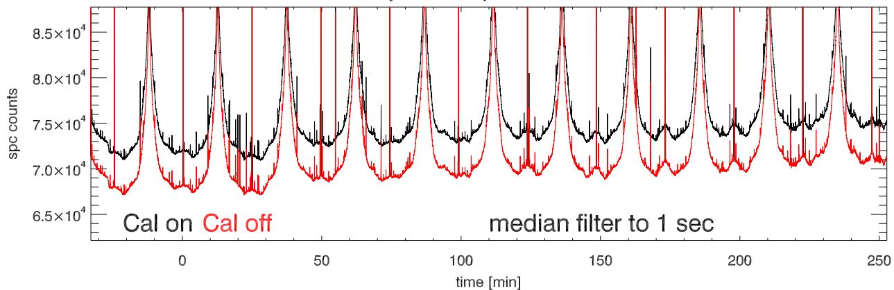
20may11 a2030 tp vs time. Beam4A
