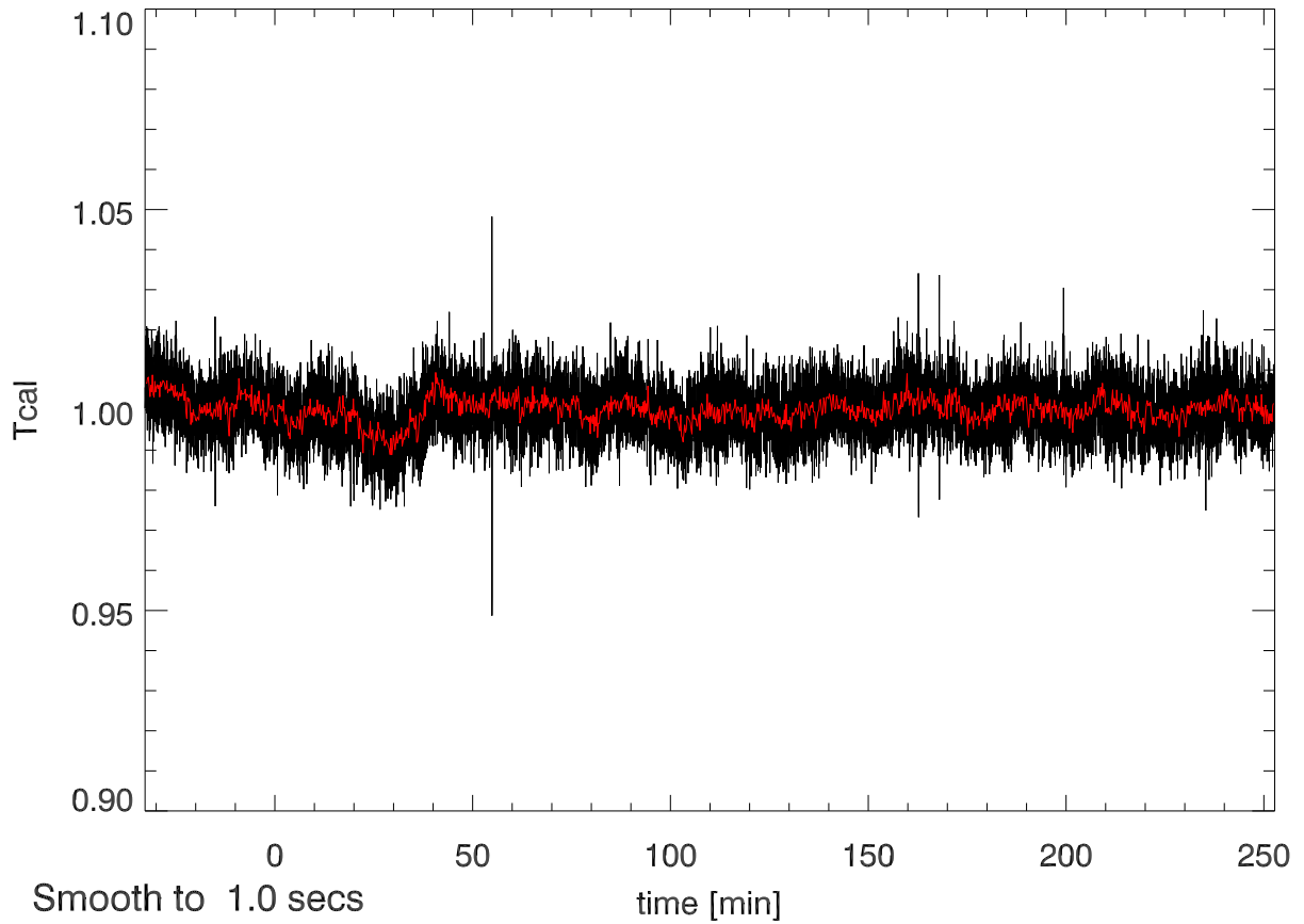
20may11 calOn - calOff Beam4A SigA: 0.011
