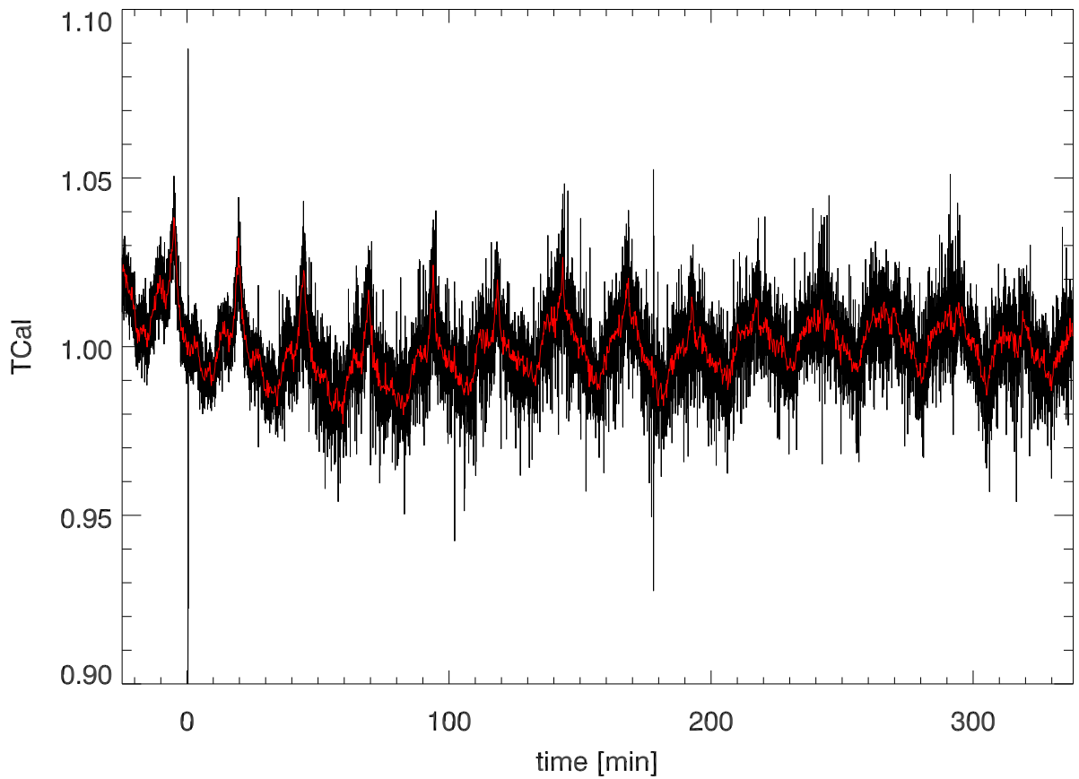
calOn - calOff Beam4B SigB: 0.015
