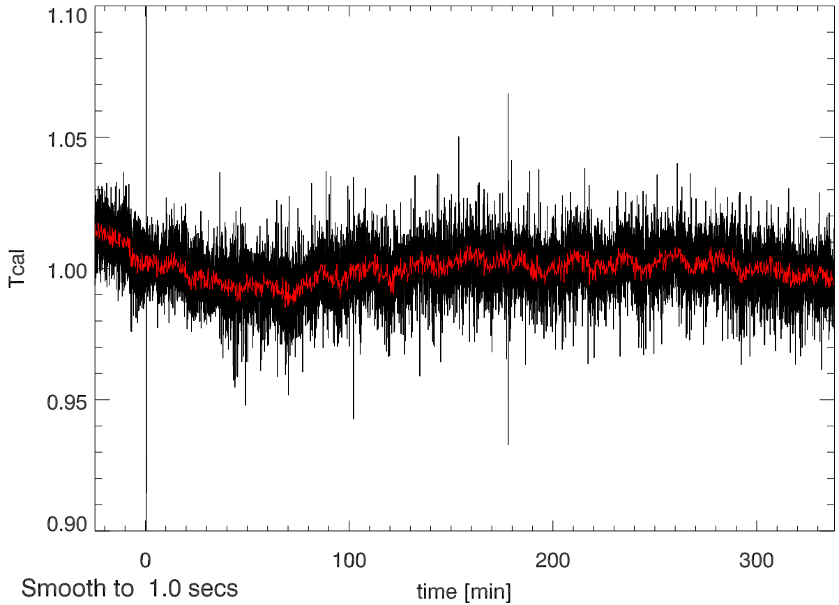
20jun12 calOn - calOff Beam4A SigA: 0.015
