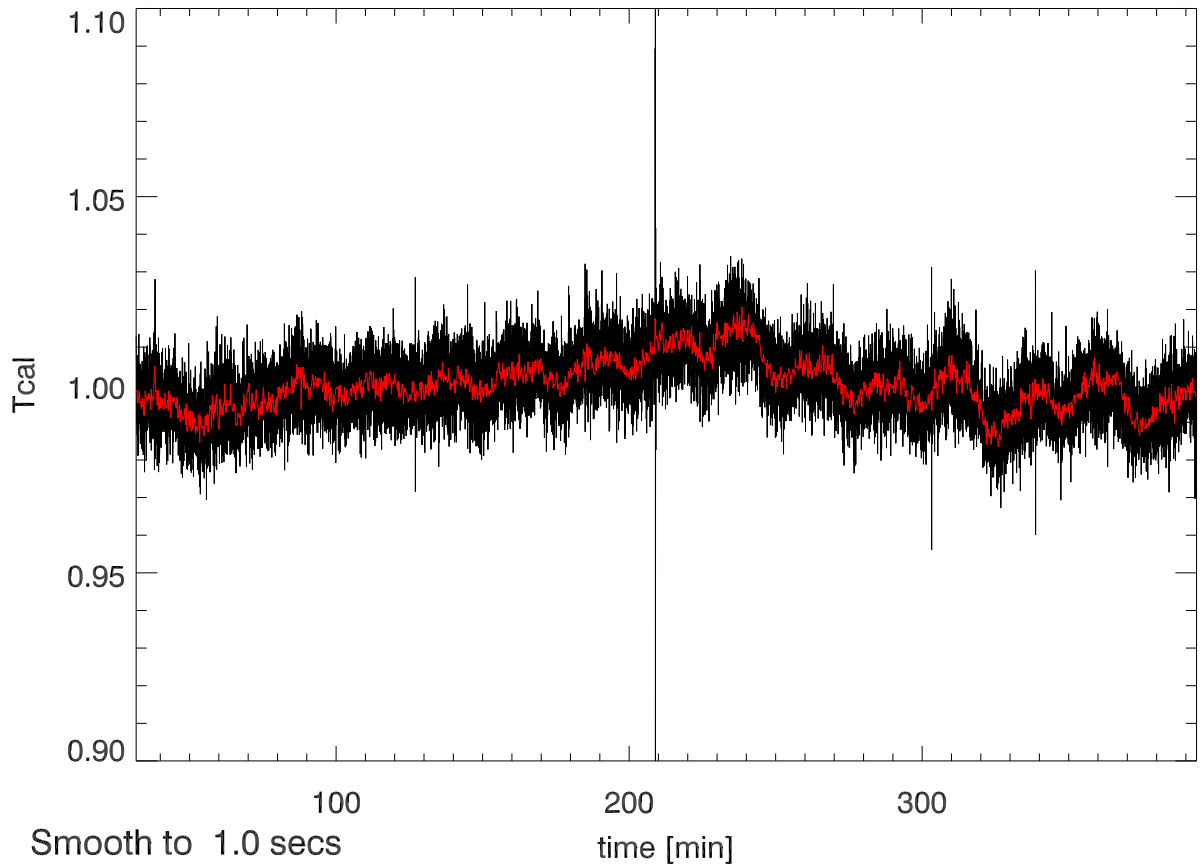
13apr11 calOn - calOff Beam4A SigA: 0.013
