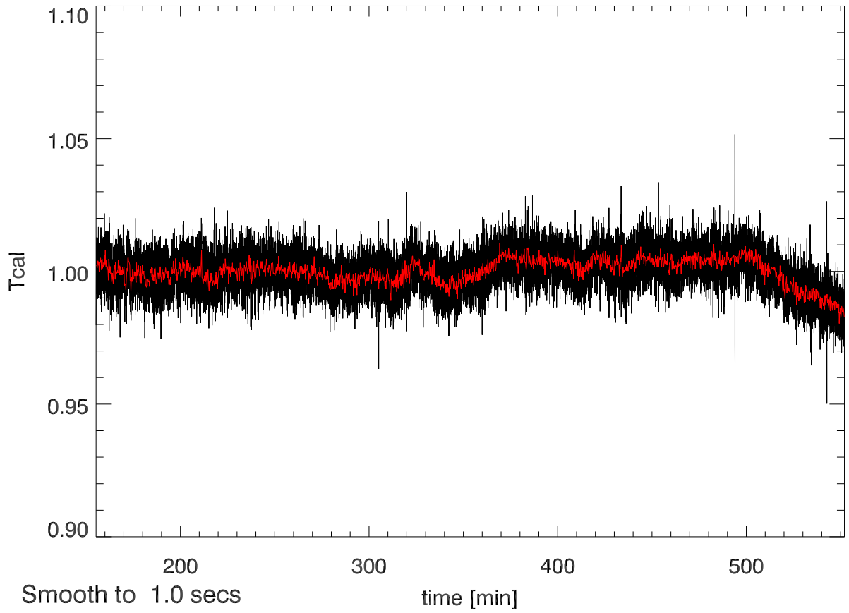
01aug12 calOn - calOff Beam4A SigA: 0.012
