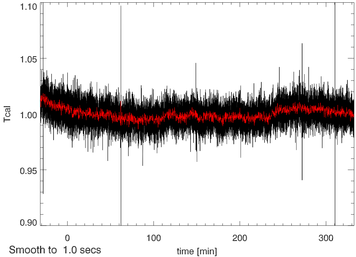
26oct11 calOn - calOff Beam3A SigA: 0.017
