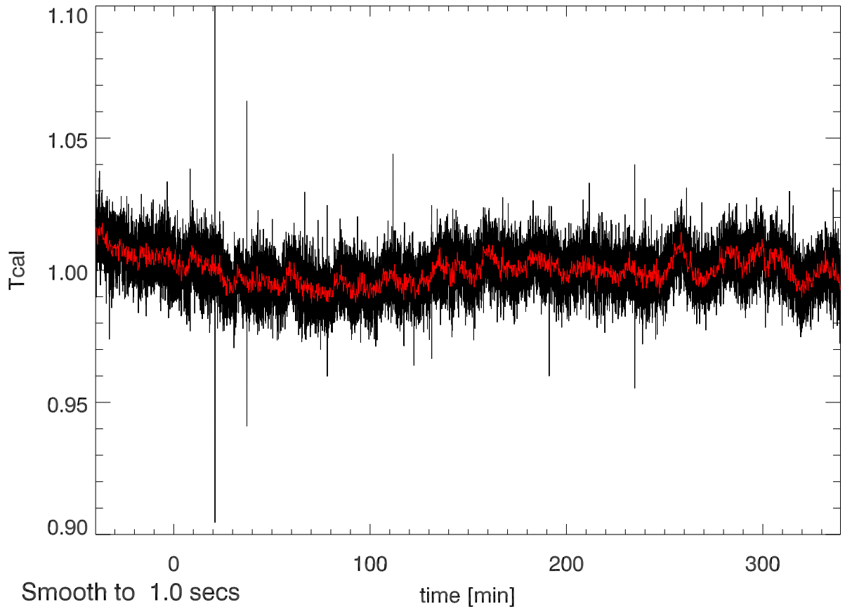
24sep12 calOn - calOff Beam3A SigA: 0.014
