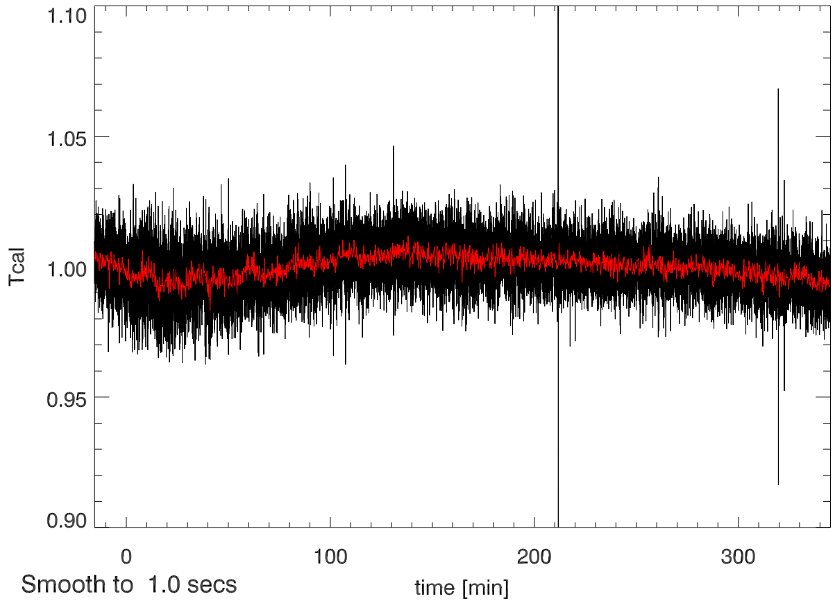
22oct11 calOn - calOff Beam3A SigA: 0.017
