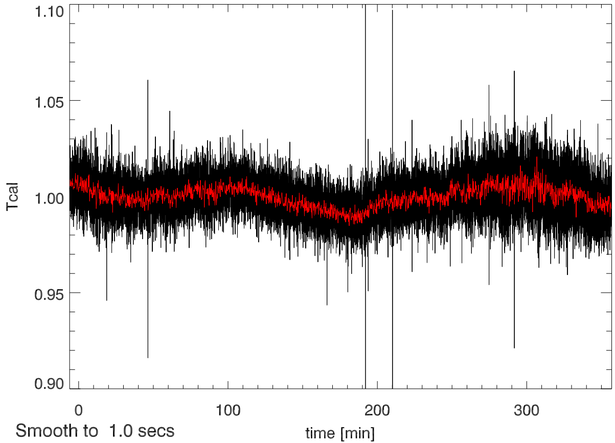
20oct11 calOn - calOff Beam3A SigA: 0.018
