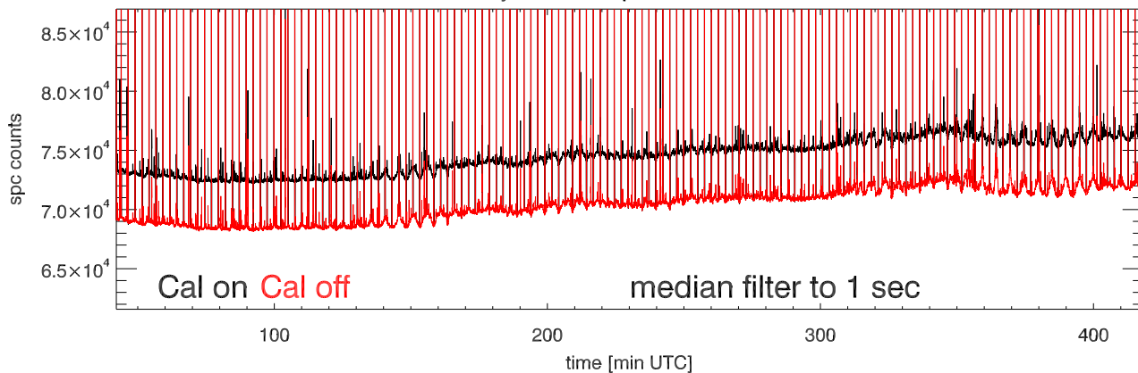
20may13 a2030 tp vs time. Beam3A
