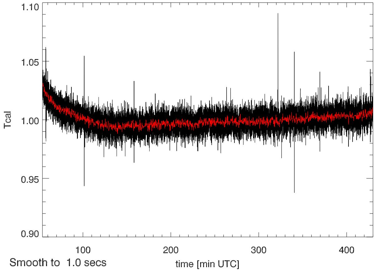
17may13 calOn - calOff Beam3A SigA: 0.013
