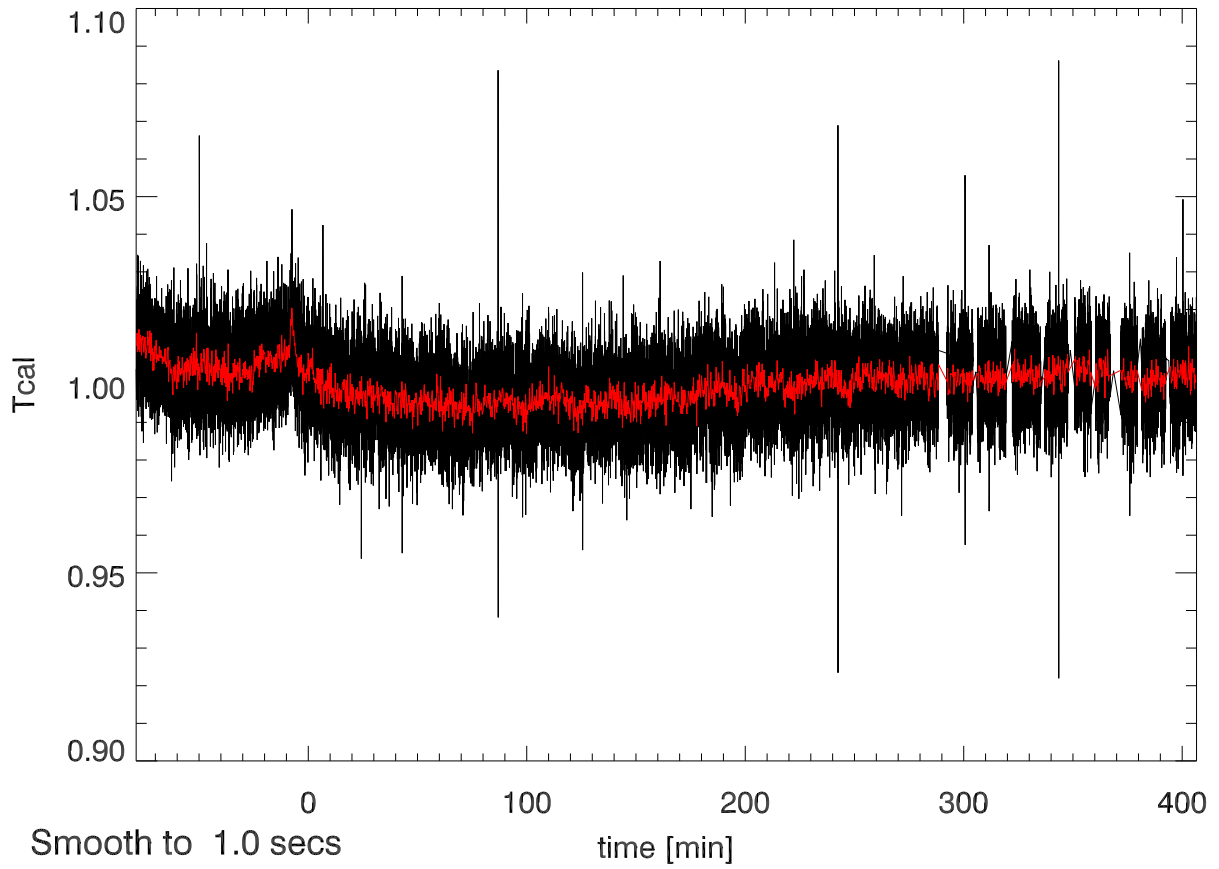
07nov11 calOn - calOff Beam3A SigA: 0.017
