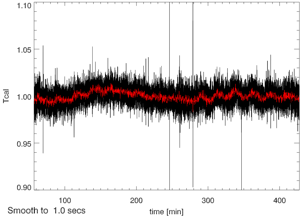
06jul11 calOn - calOff Beam3A SigA: 0.016
