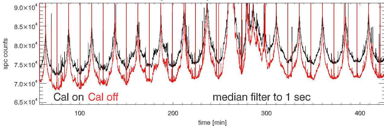
06jul11 a2030 tp vs time. Beam3A
