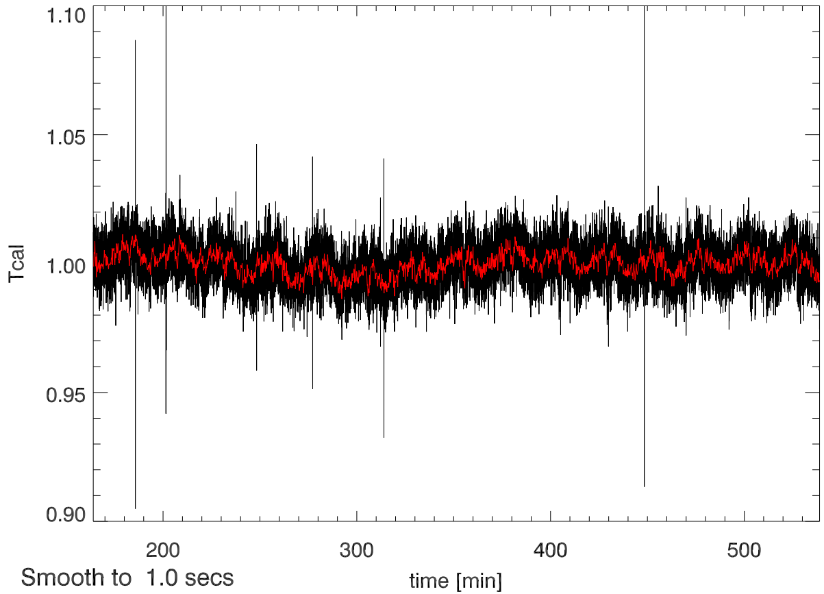
03feb13 calOn - calOff Beam3A SigA: 0.013
