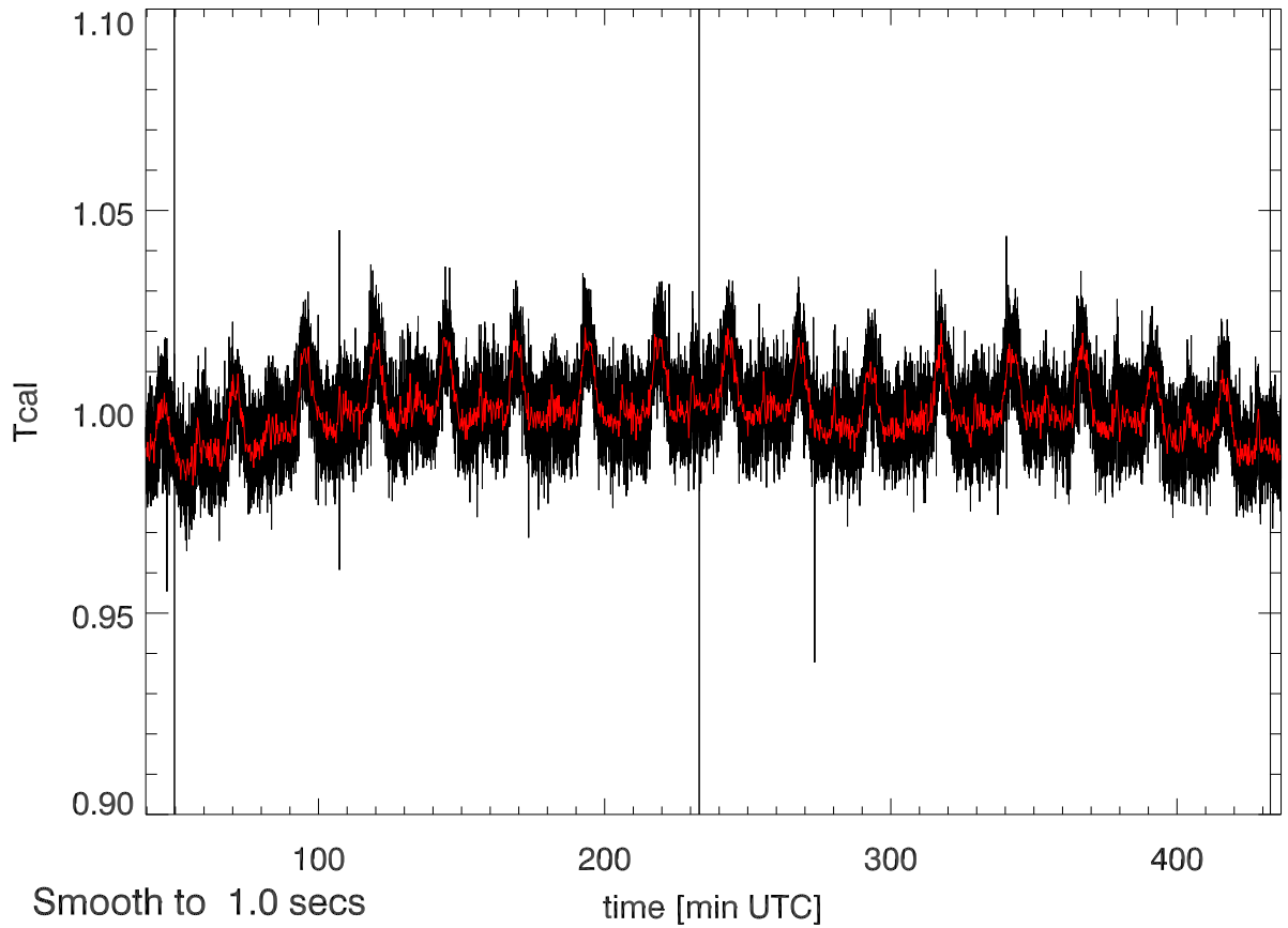
01mar13 calOn - calOff Beam3A SigA: 0.014
