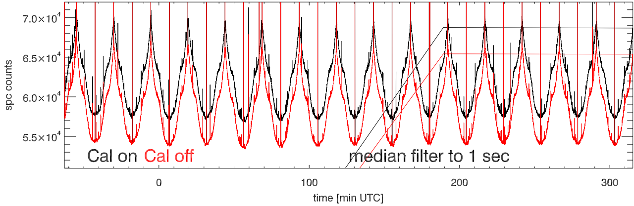
31mar13 a2030 tp vs time. Beam2A
