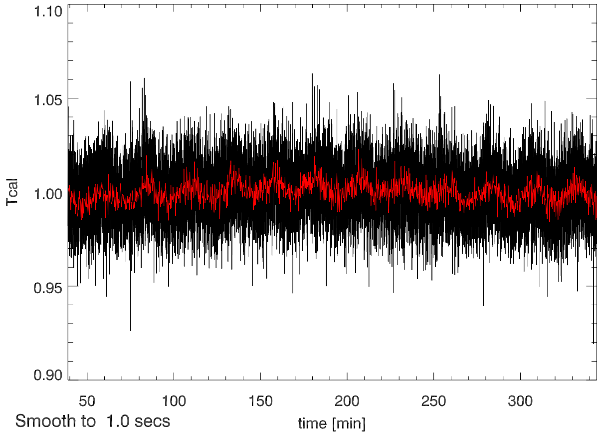
27apr11 calOn - calOff Beam2A SigA: 0.027
