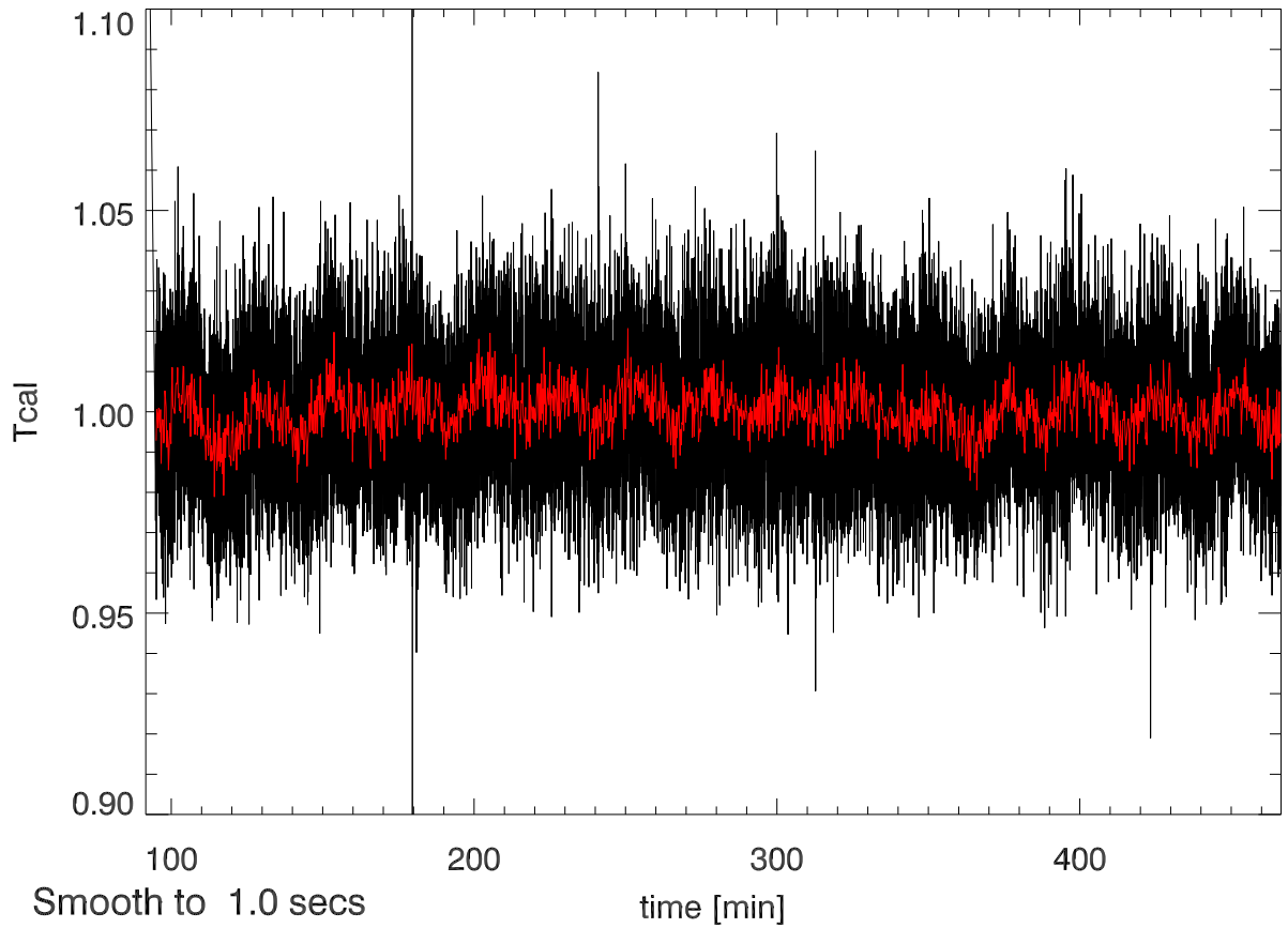
26jun11 calOn - calOff Beam2A SigA: 0.029
