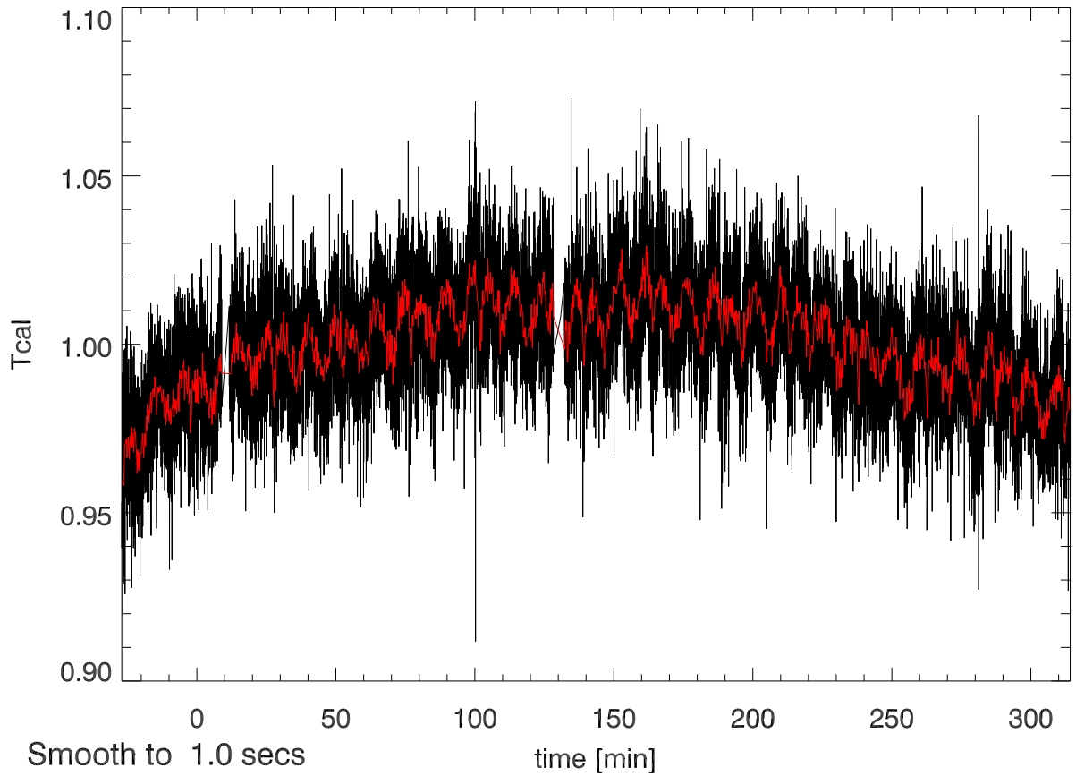
25jun12 calOn - calOff Beam2A SigA: 0.027
