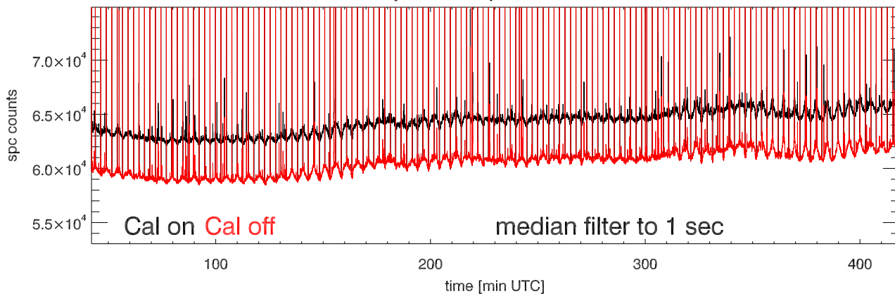
20may13 a2030 tp vs time. Beam2A
