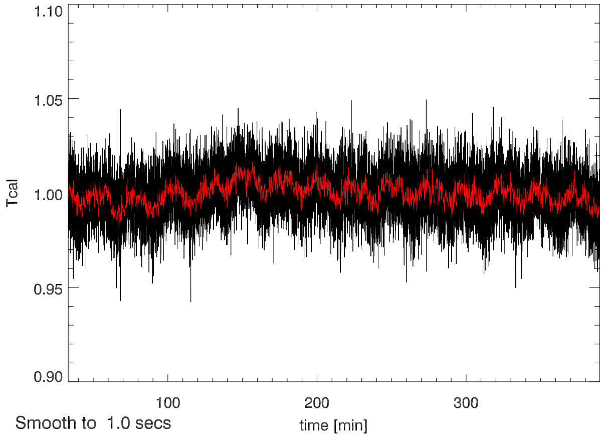
13oct11 calOn - calOff Beam2A SigA: 0.022
